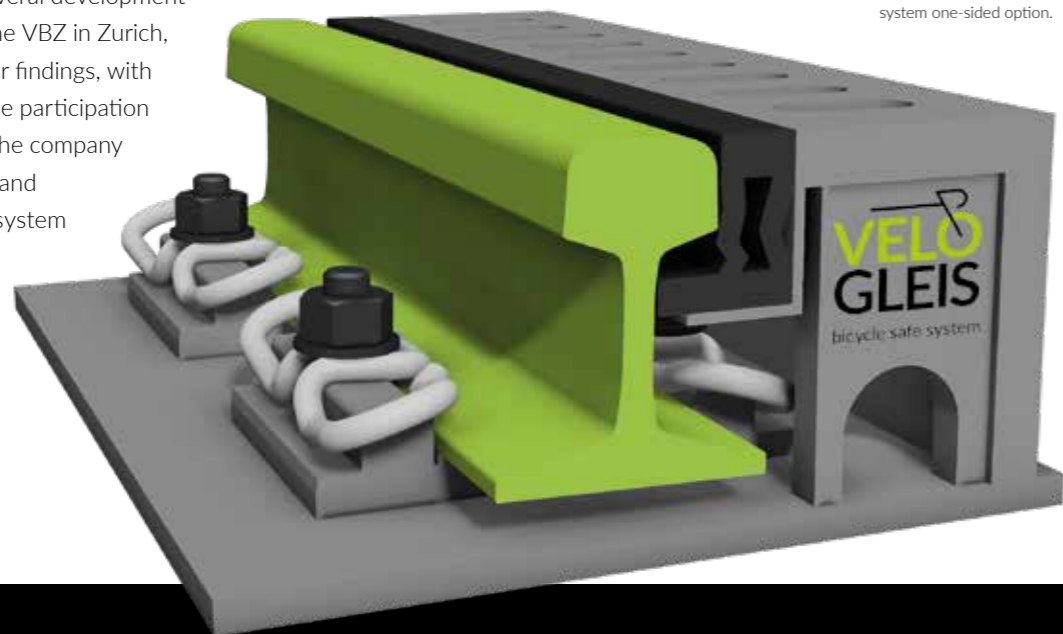
3D view of the patented SEALABLE VeloGleis box construction system one-sided option.
